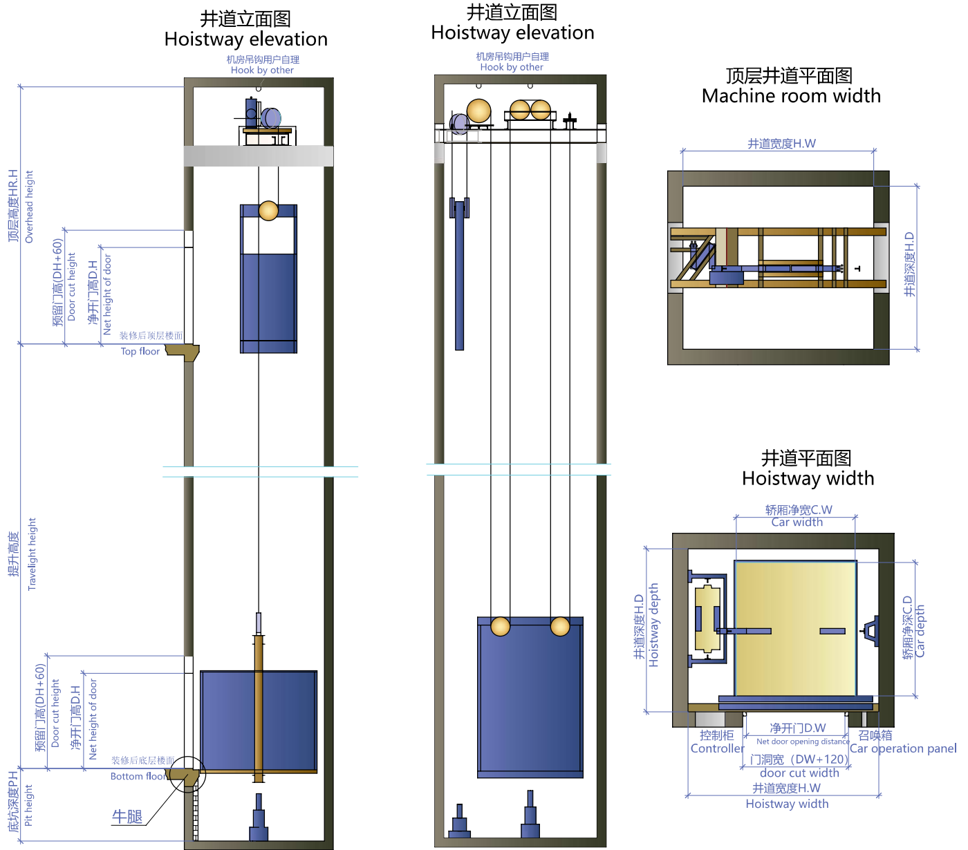
HD-F30 系列无机房载货电梯参数表 HD-F30 series roomless freight elevator Specifications
